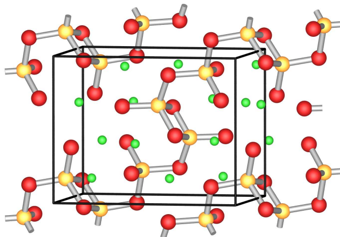
\text{Na}_7\text{In}_3\text{Se}_8
